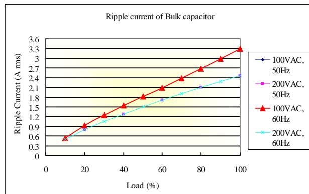
Fig. 4 Bulk cap ripple current requirement vs. Output load
