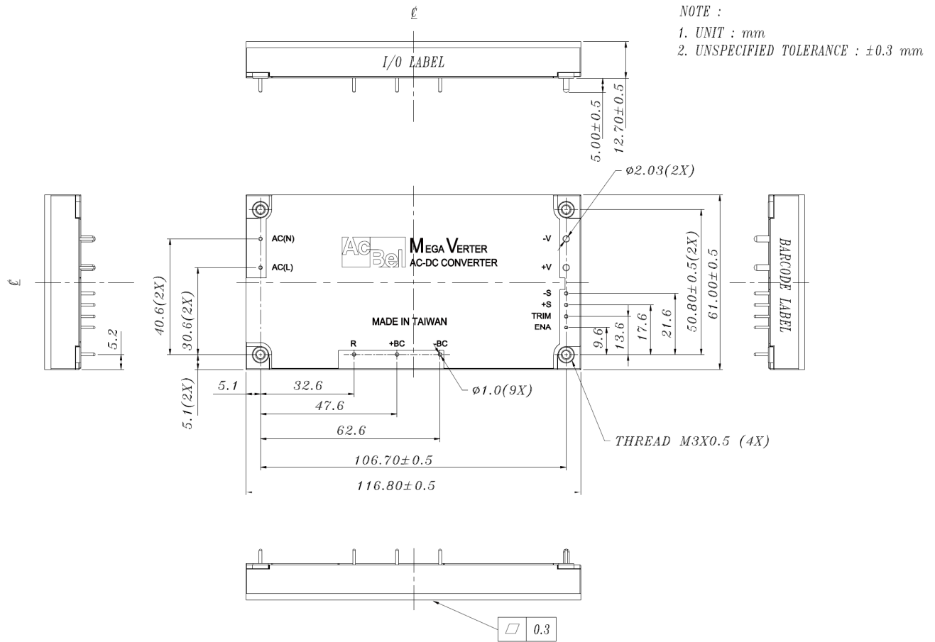
Fig. 6 Outline drawing.
