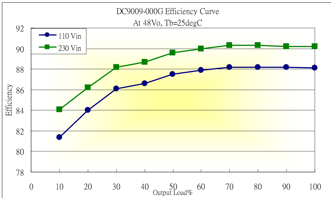
Fig. 5 Efficiency curve.
