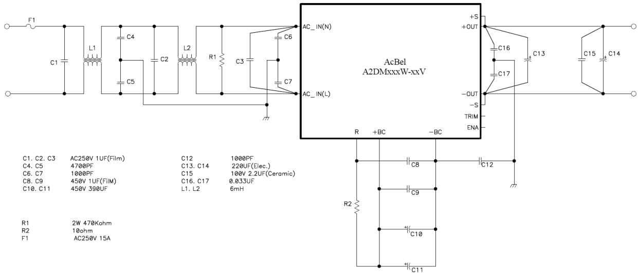
Fig. 3 Application Circuit.
