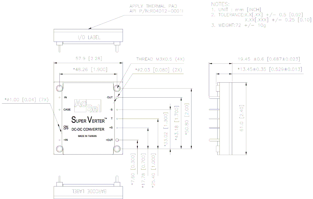
Fig. 7 Outline Drawing
