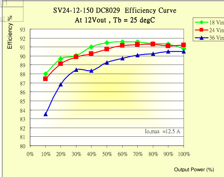
Fig. 4 Efficiency Curve
