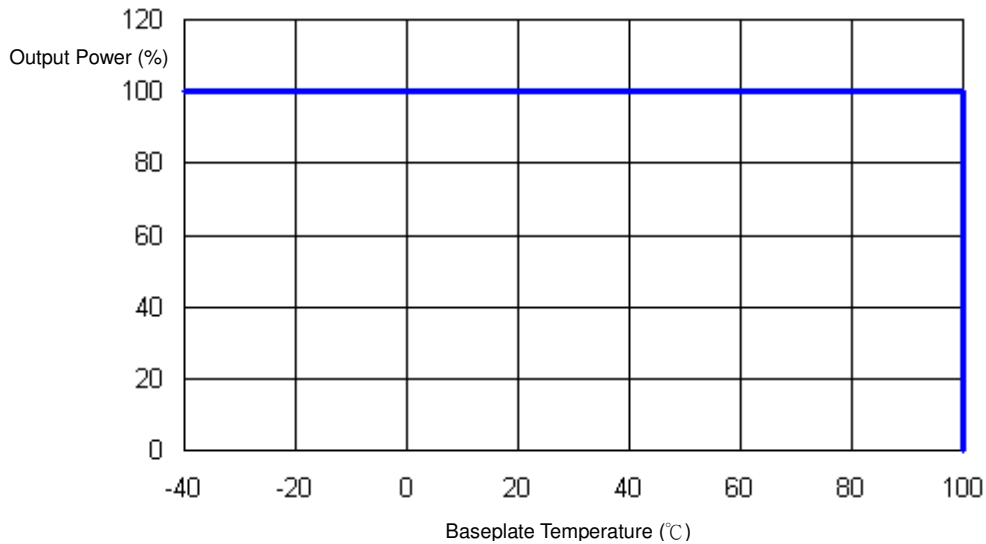
Fig. 5 Derating Curve
