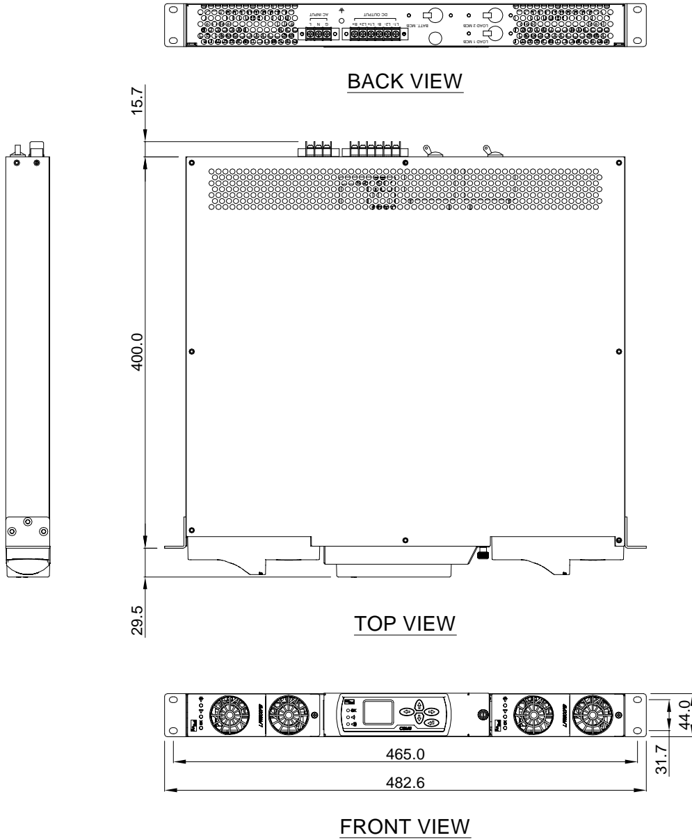
Fig 1. Outline Drawing of HR8057-001
